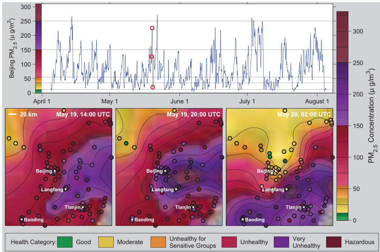
Figure 2. Time evolution of PM 2.5 pollution in the vicinity of Beijing. (Top) Time series of PM 2.5 concentration at Beijing extracted from the interpolated field. Red circles indicate times shown in bottom row. (Bottom) Maps of interpolated PM 2.5 concentration during a period of high pollution. Pollution concentrations were computed as described in the text from hourly data and maps were rendered in MATLAB. Concentrations are shown using color gradients and contour lines, where color tones (green, yellow, etc.) correspond to health impact categories defined by the US EPA. Bold circles show station locations with the observed value at each station indicated by the color within the circle.
